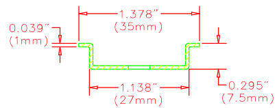
FRONT SECTION
